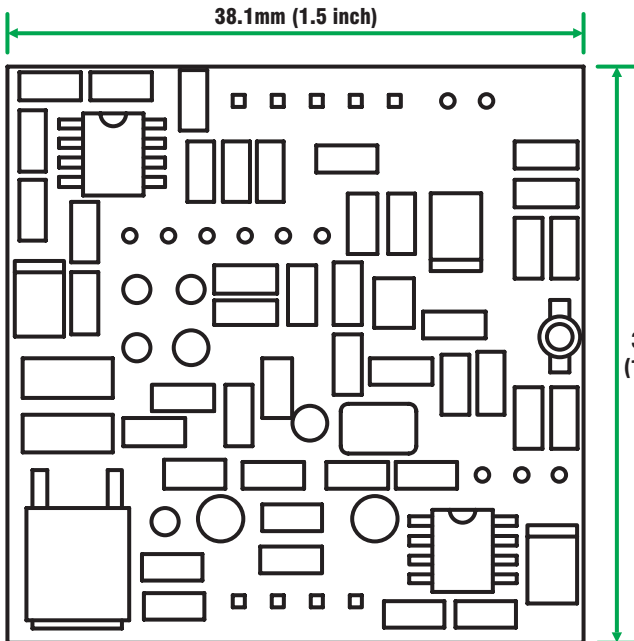
2:1 TOP VIEW
