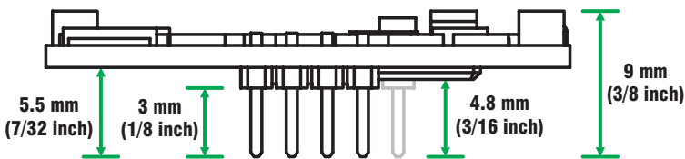
2:1 SIDE VIEW
